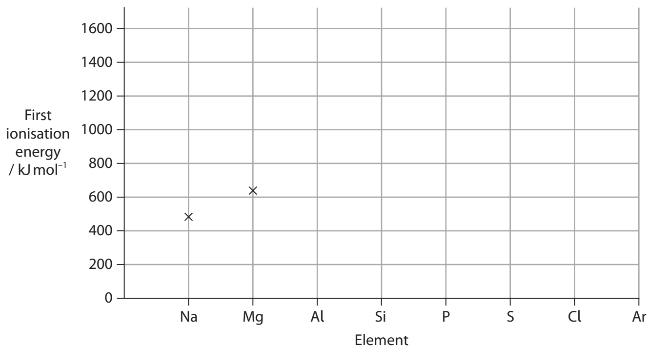
First ionisation energies of the Period 3 elements
